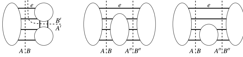
Figure 10: Cyclic 4-edge-cuts containing e if i_0 = k .
