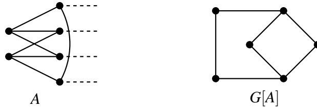
Figure 8: The exceptional graph of Lemma 23.
