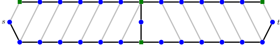
Figure 3: Example showing that the computed connected- T -join is not necessarily shorter than \frac{3}{2} times the optimum. For each k \in \mathbb{N} , we have a graph G with 8k + 5 vertices and 12k + 5 edges. Two vertices are labeled s and t ; they form the set T = \{s, t\} . The figure shows the case k = 3 . Note that there is a Hamiltonian s - t -path, and hence \text{LP}(G, T) = \text{OPT}(G, T) = 8k + 4 . Also note that \varphi(G) = 2 because G is not factor-critical. Suppose that we choose the ear-decomposition that begins with the circuit of length 8k + 4 and then has one pendant 2-ear (in the center). Then \pi = 1 = \frac{1}{2}\varphi(G) , so we have two choices in our algorithm. If we use Theorem 24, then our algorithm first takes the 2-ear and then adds edges to obtain a spanning tree, e.g., the one with thick edges. Then there are four vertices (shown as squares) whose degrees have the wrong parity, and we need another 4k + 2 edges to correct the parities. So we end up with a connected- T -join with 12k + 6 edges. If we use Proposition 8 instead, we could also end up with 12k + 6 edges.
