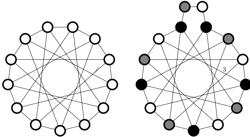
FIG 1. Graphs R_{3,5} and G_{5,8}
